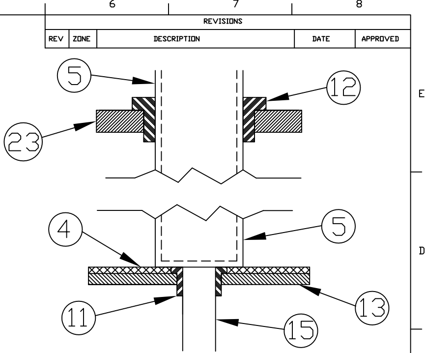
Bearing Detail
